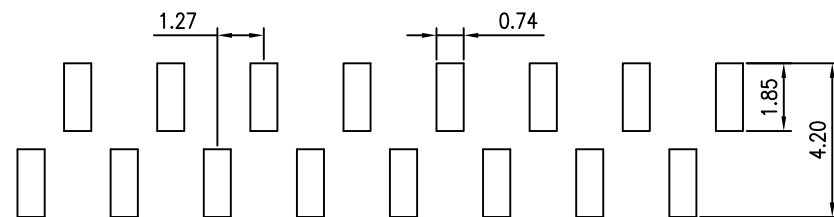
P.C.B LAYOUT (SMT A Type)
