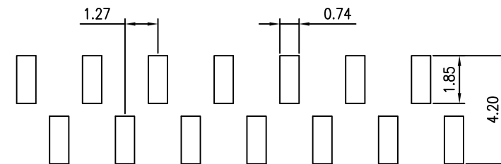
P.C.B LAYOUT (SMT B Type)
