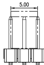
2x2~2x3Pin (CAP)
