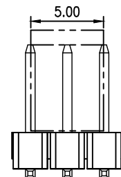
2x2~2x3Pin (CAP)
